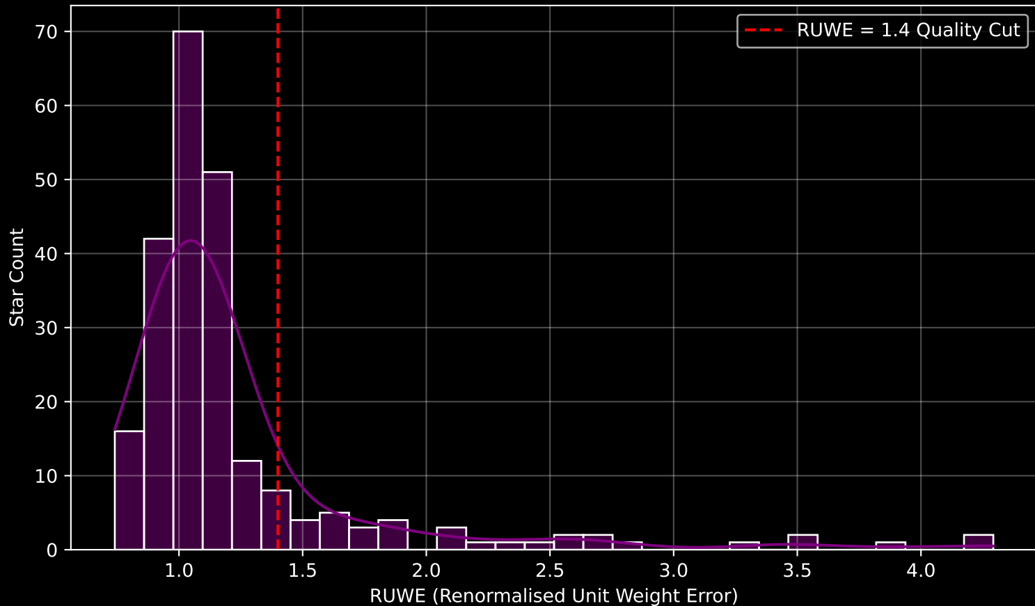
GALAH DR4 Field [7131] RUWE Distribution (n= 232)
