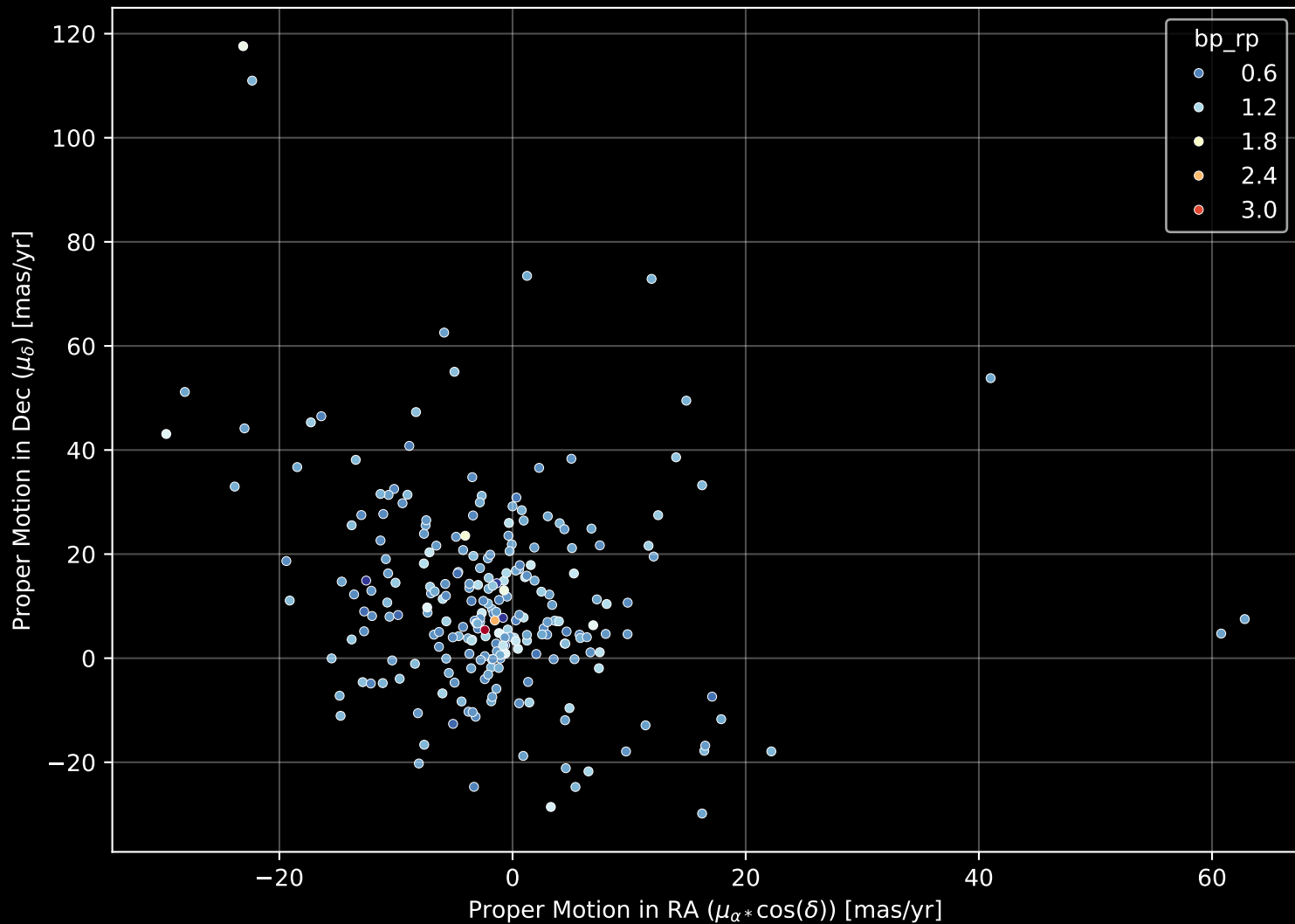
GALAH DR4 Field: [7131] Proper Motion Diagram (n= 243)
